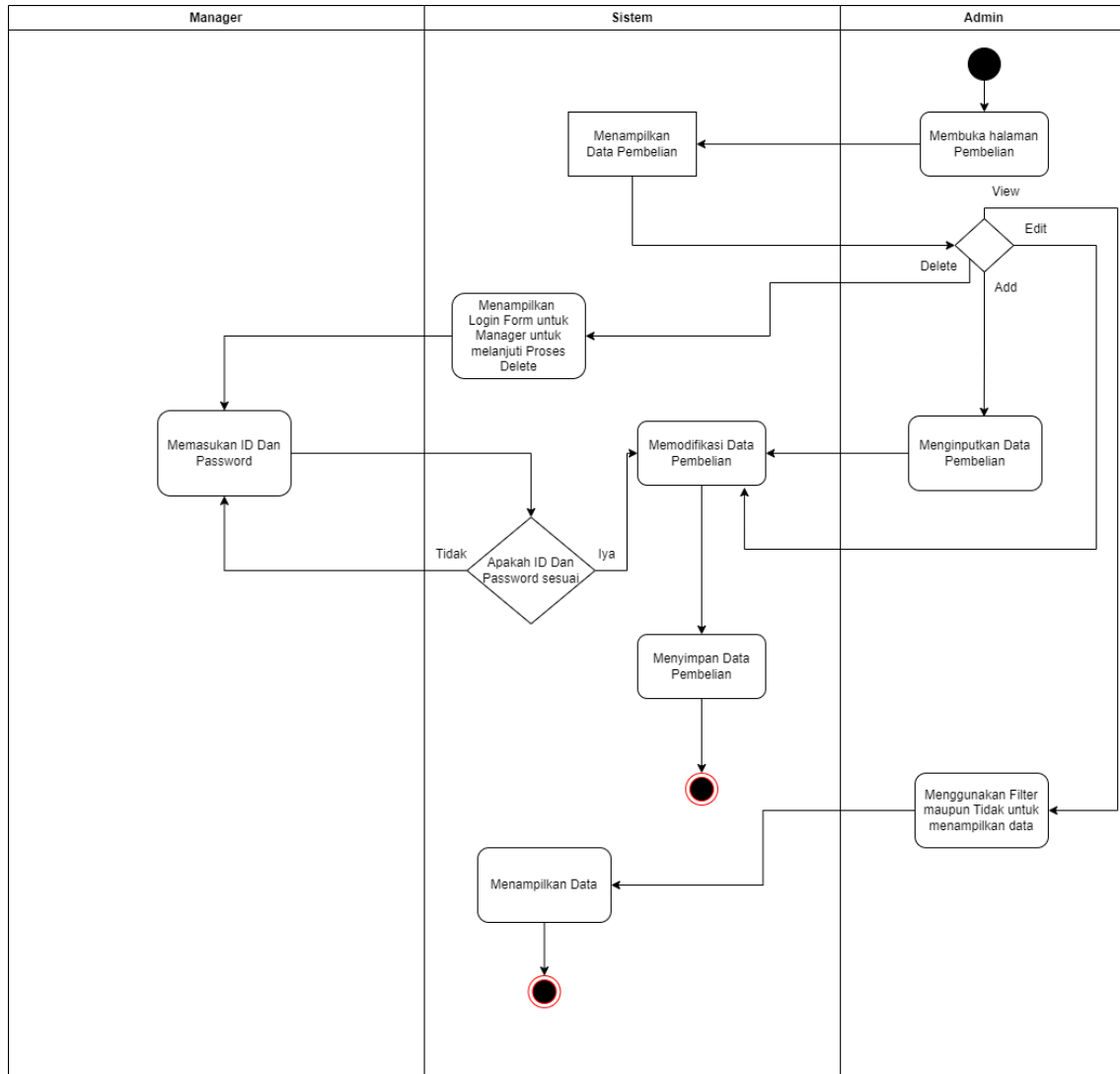
Gambar 3.10 Activity Diagram Pembelian
