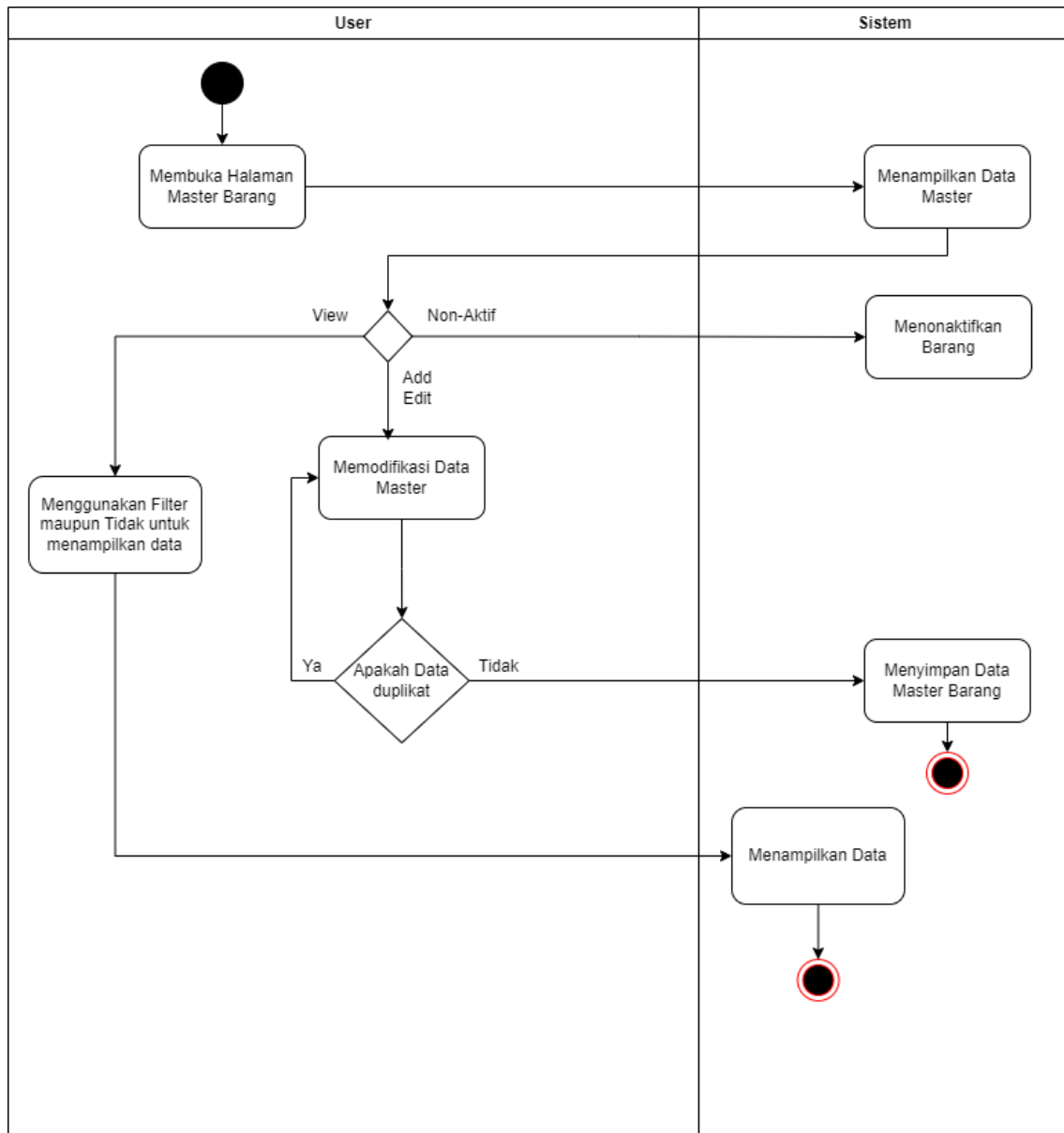
Gambar 3.8 Activity Diagram Master Barang
