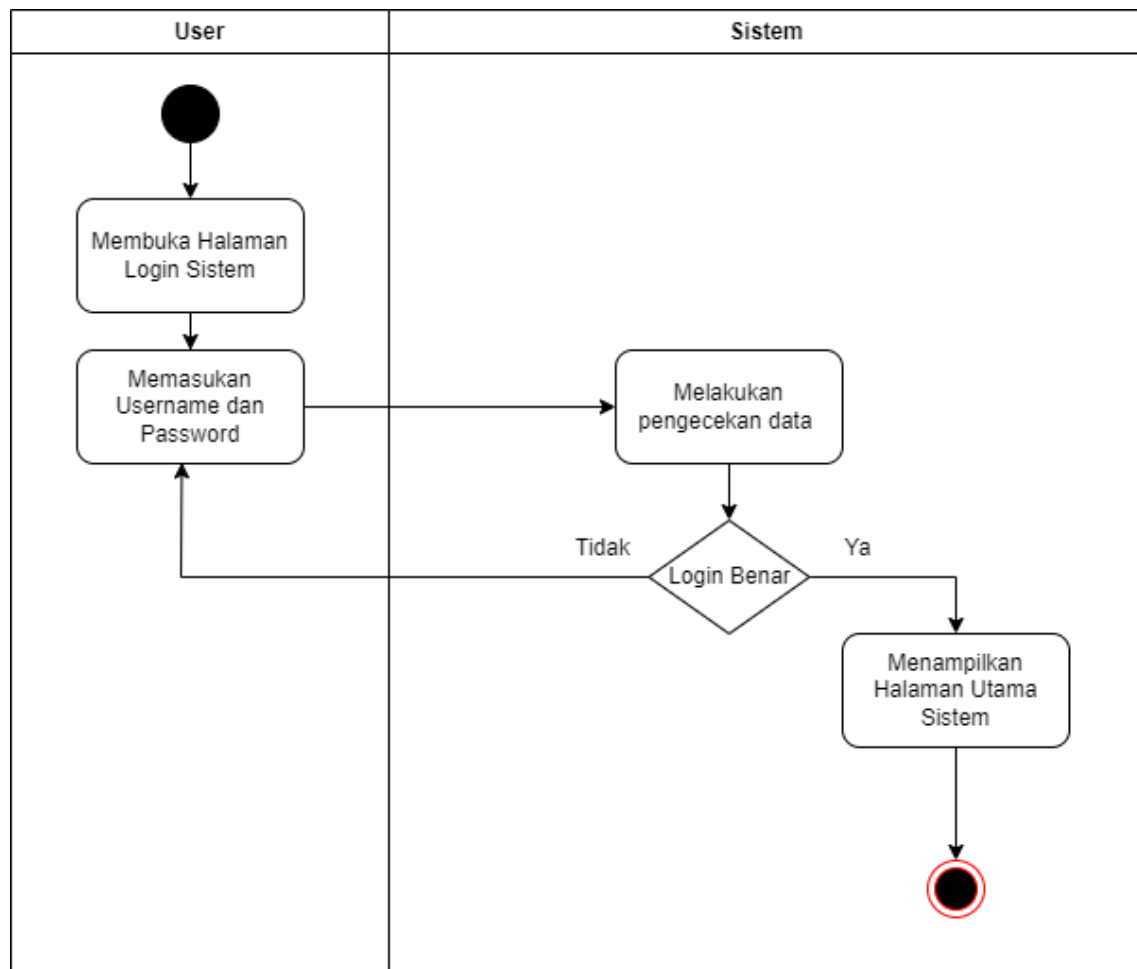
Gambar 3.1 Activity Diagram Login
