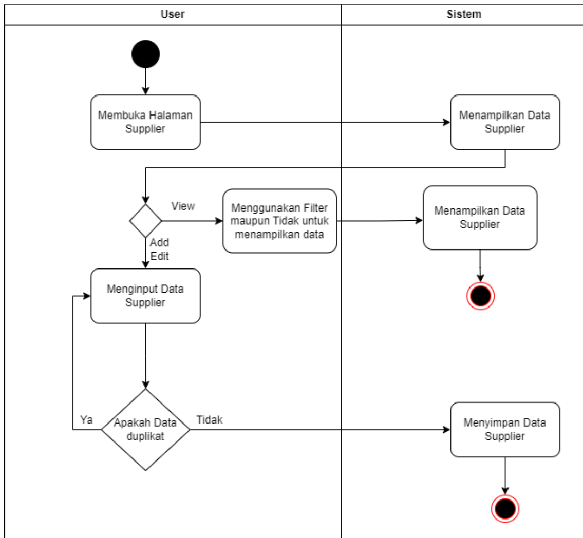
Gambar 3.2 Activity diagram Supplier
