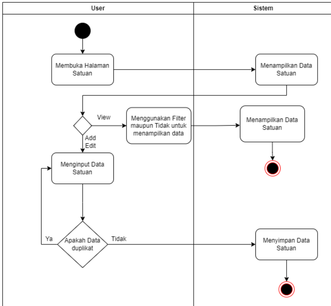
Gambar 3.7 Activity Diagram Master Satuan
