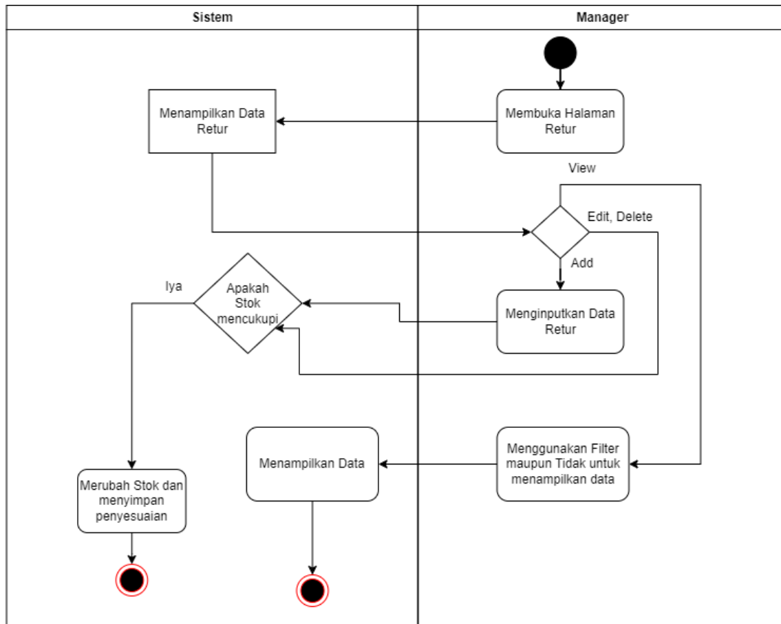
Gambar 3.14 Activity Diagram Retur
