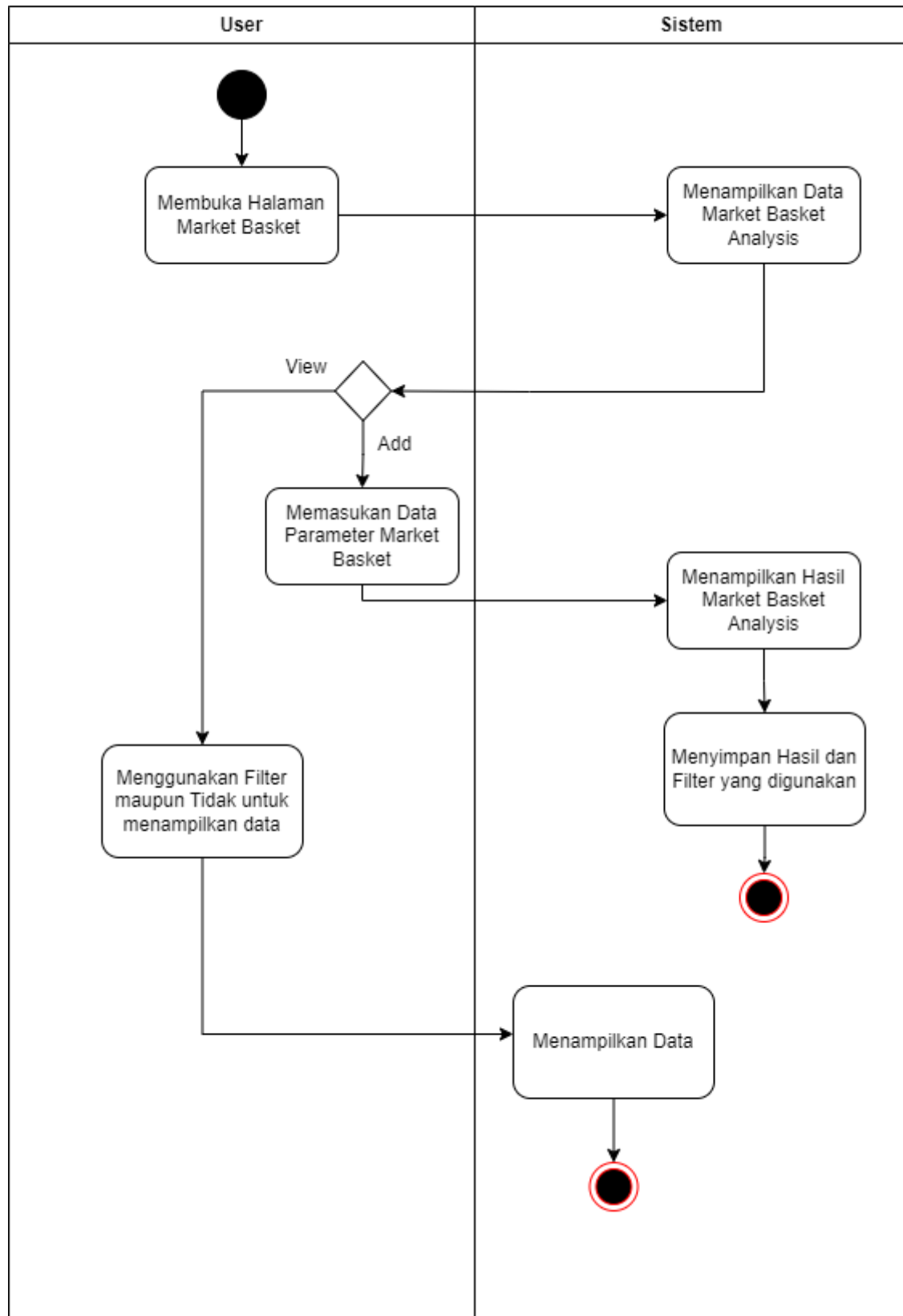
Gambar 3.15 Activity Diagram Market Basket Analysis
