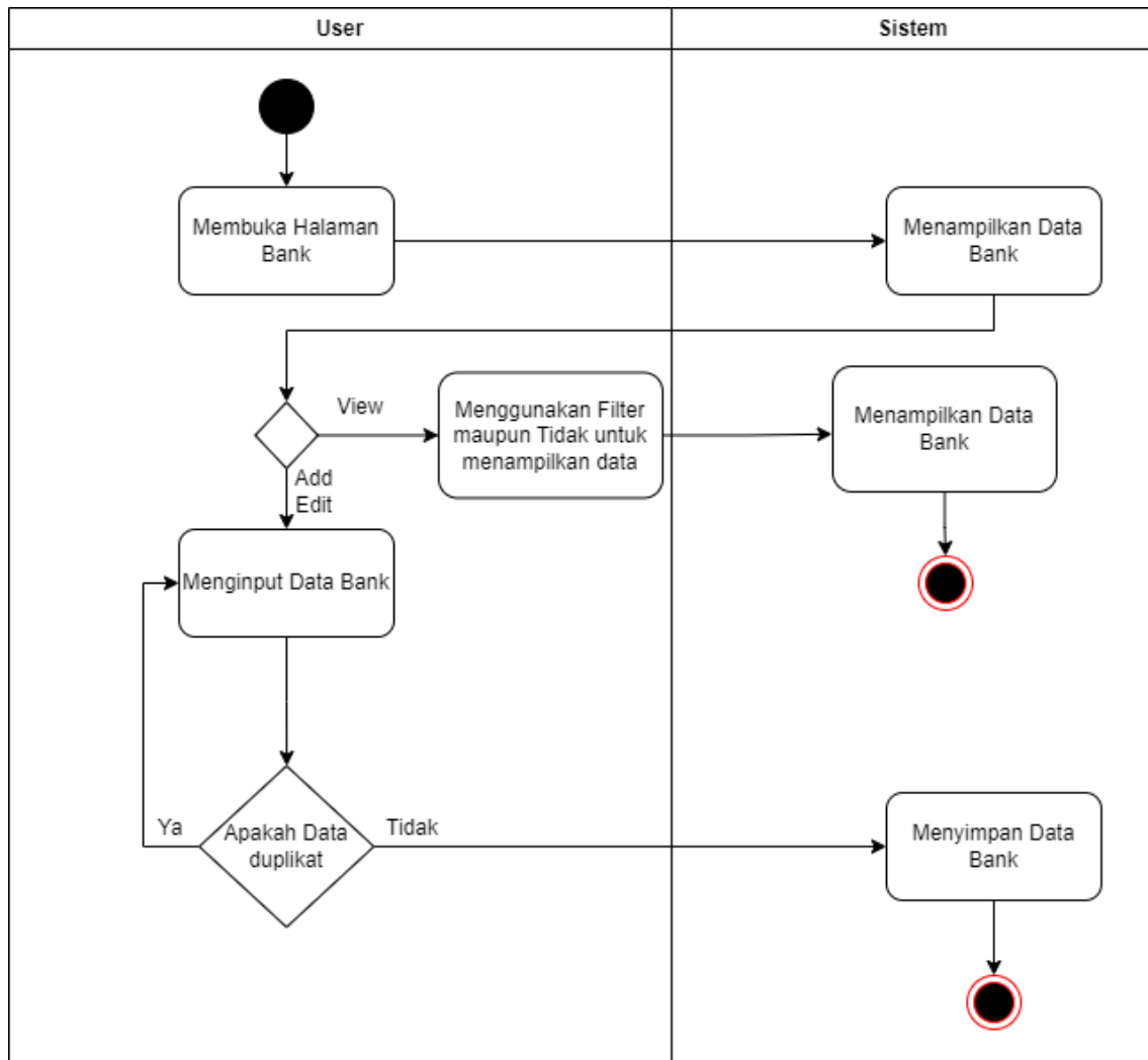
Gambar 3.5 Activity Diagram Master Bank
