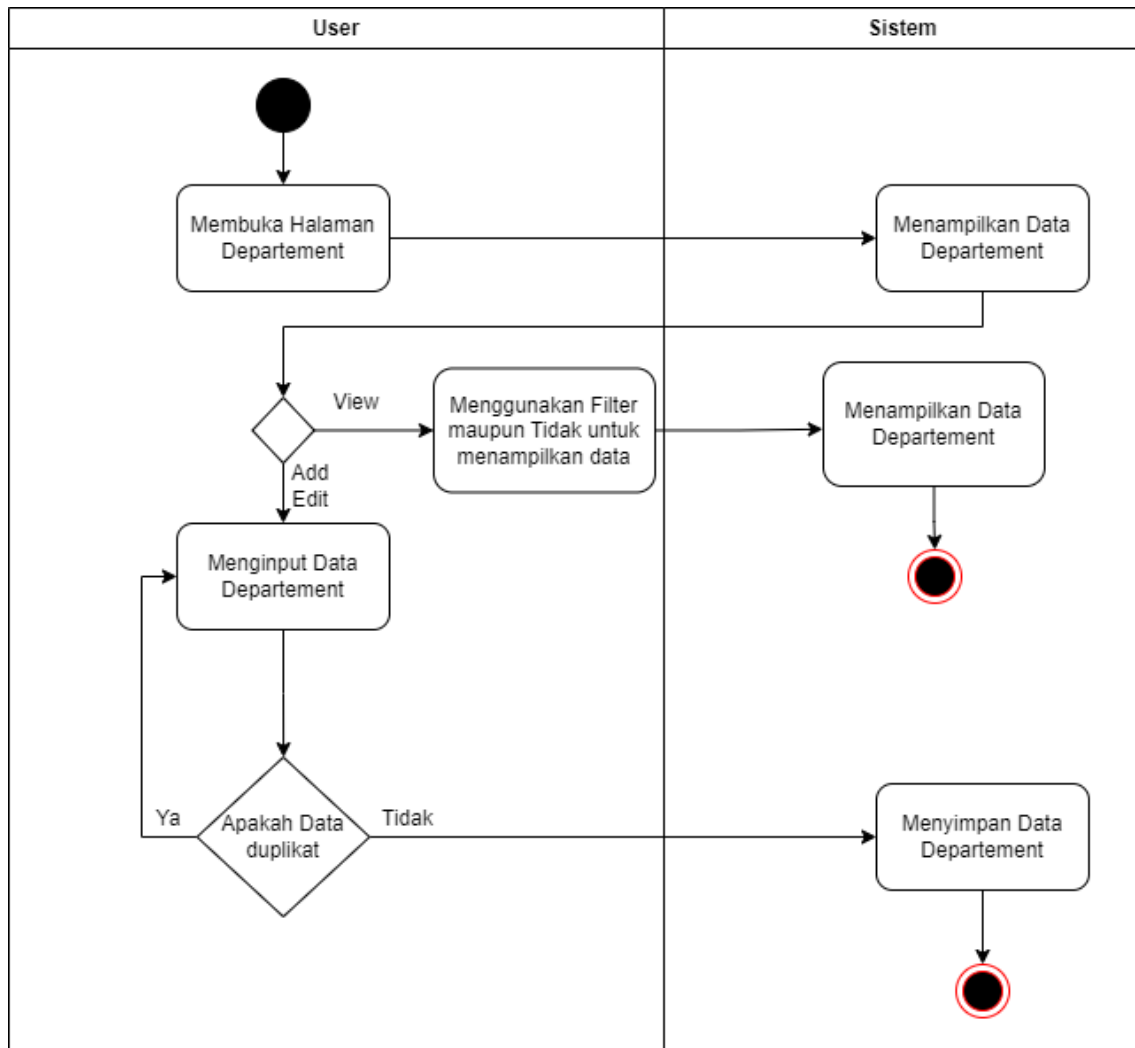
Gambar 3.6 Activity Diagram Master Departement
