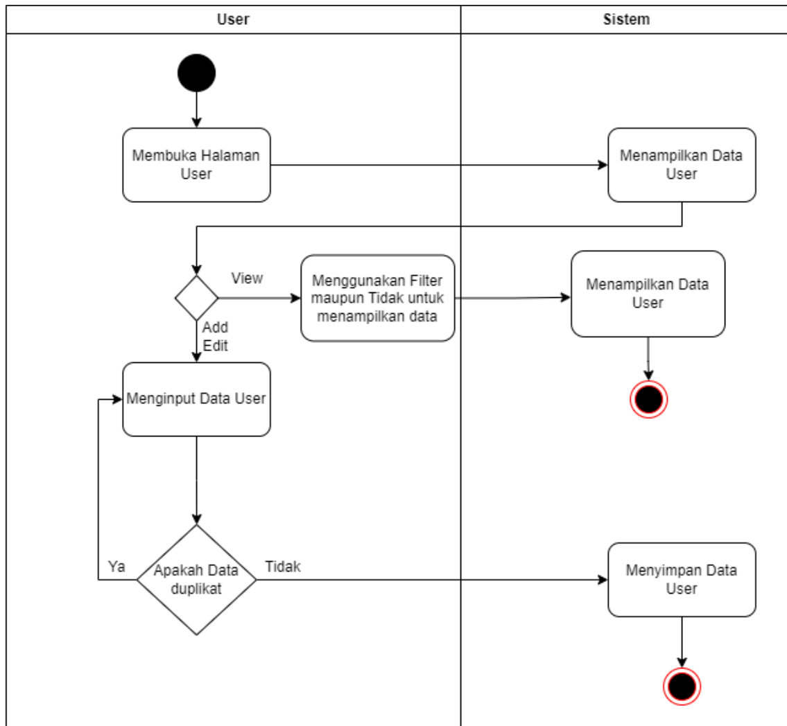
Gambar 3.3 Activity Diagram User
