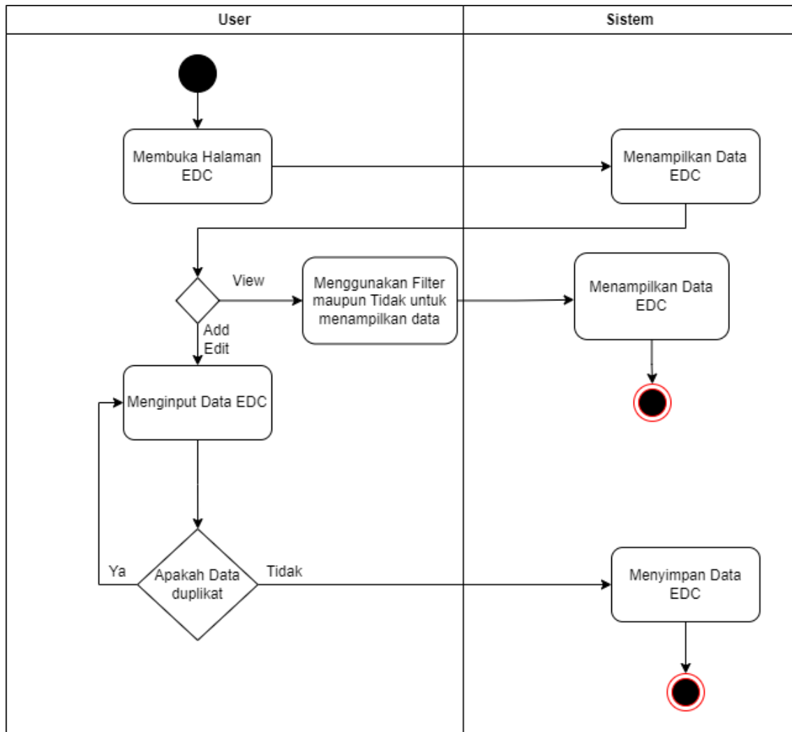
Gambar 3.4 Activity Diagram Master EDC
